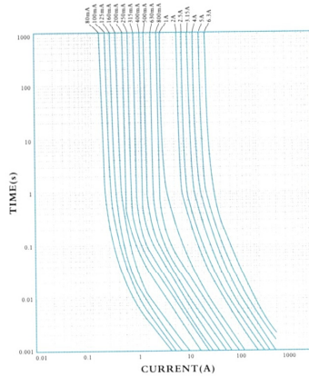
I-T CHARACTERISTICS CURVE
