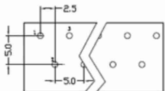
PCB B Type
