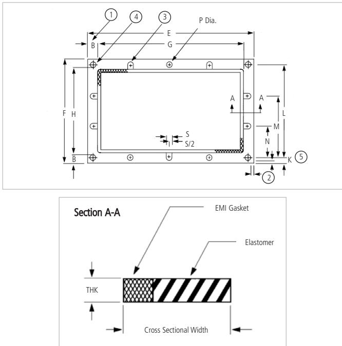
FIGURE 2. ENVIRO-SEAL GASKET
