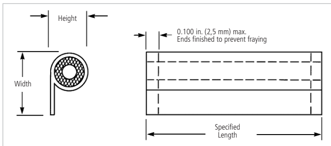
FIGURE 2. CUT-TO-LENGTH
