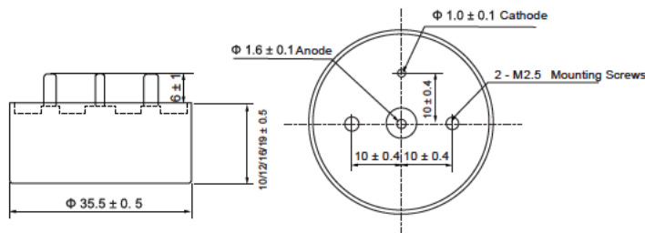
Mounting Dimensional Diagram of HTHC2W Φ35.5 x 10/12/16/19 (Type A)
