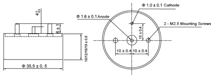
Mounting Dimensional Diagram of HTHC2W Φ35.5 x 10/12/16/19 (Type B)
