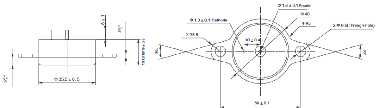
Mounting Dimensional Diagram of HTHC2FB \Phi 35.5 \times 10/12/16/19
