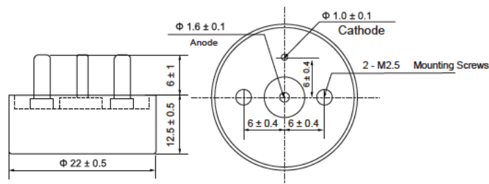
Mounting Dimensional Diagram of HTHC1W \Phi 22 \times 12.5
