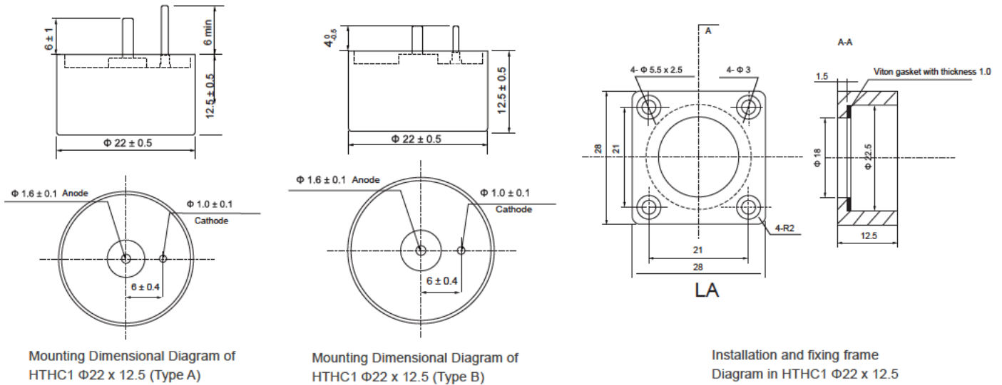
Figure 2 Outline Structure and Mounting Dimensional Diagram
