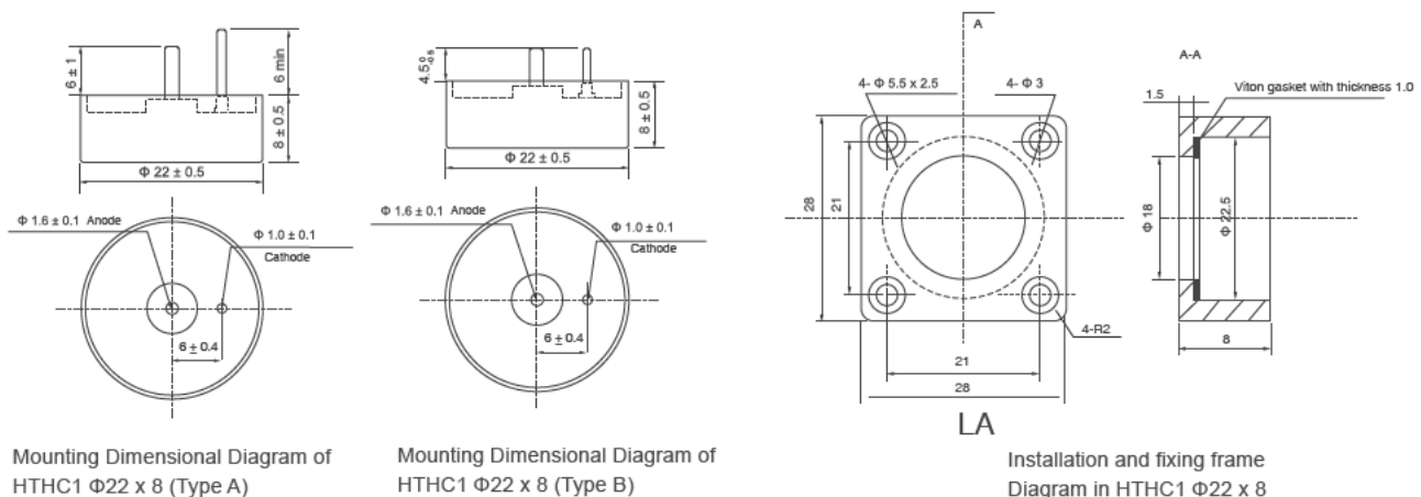
Figure 1 Outline Structure and Mounting Dimensional Diagram
