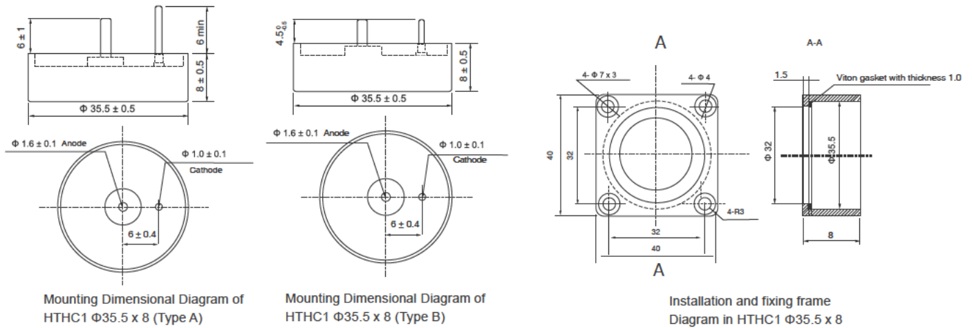
Figure 3 Outline Structure and Mounting Dimensional Diagram
