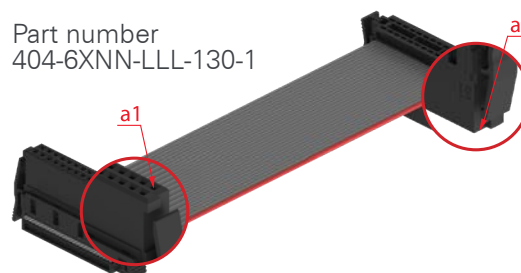
Assembled version 130
