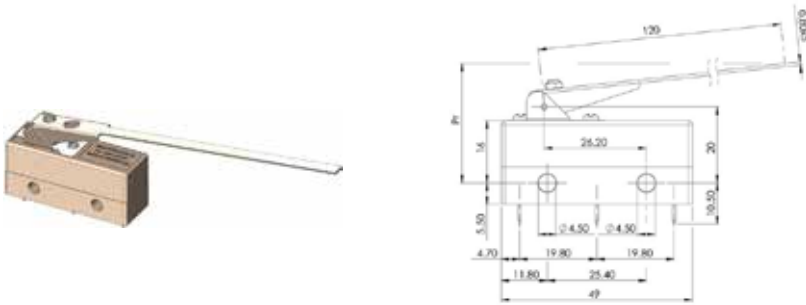
Type 7A120 : Simple Long Adjustable Lever - Direct Action -
