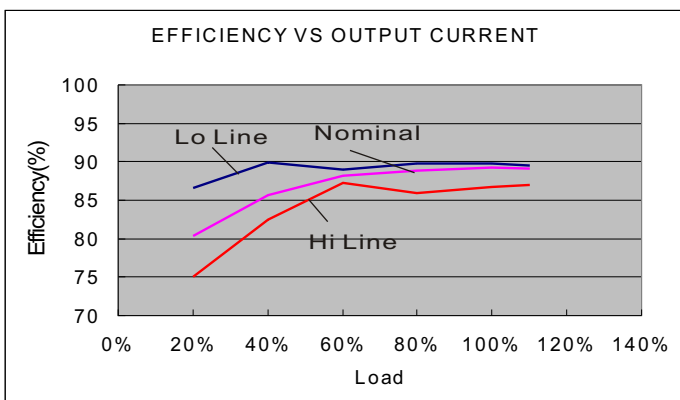
SU-4815S12
