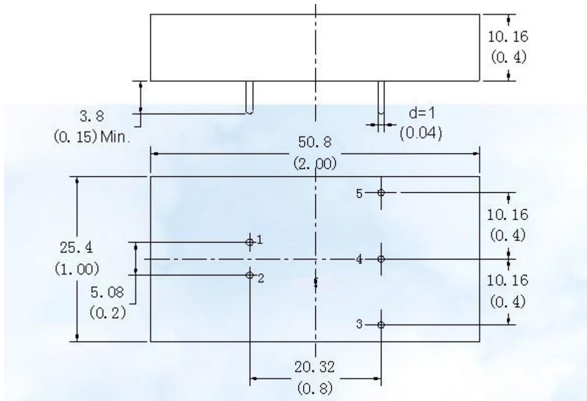
BOTTON VIEW
