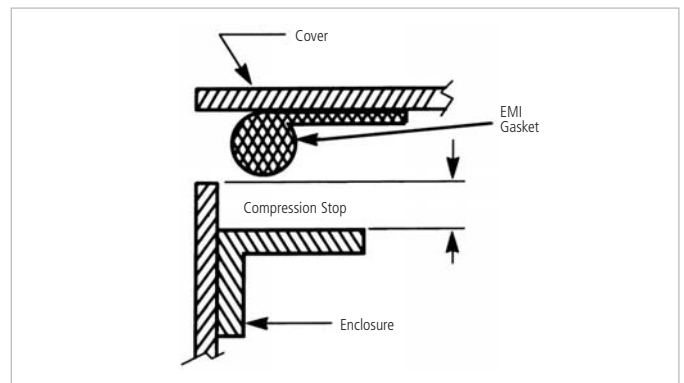
FIGURE 5B. COMPRESSION STOP BUILT INTO ENCLOSURE
