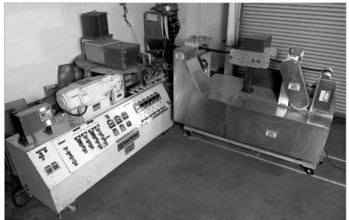
Thermoplastic extruder for microwave absorbing thermoplastic products.
