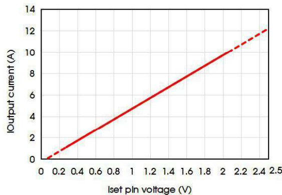
Iset pin voltage VS Output current
