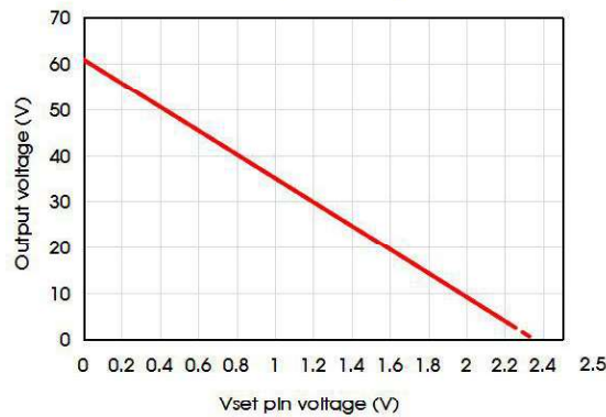
Vset pin voltage VS Output voltage
