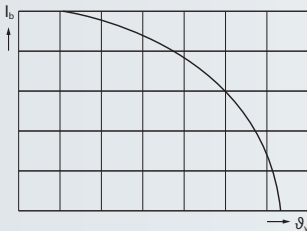
Derating-Diagramm
