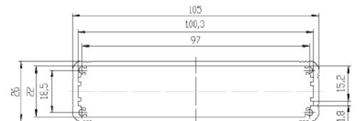
Cross section of Extrusion Microbox 36
