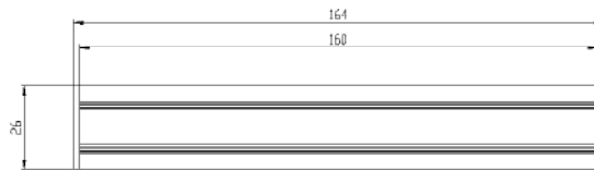
Side view Microbox 36
