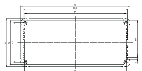
Cross section of Extrusion Microbox 36
