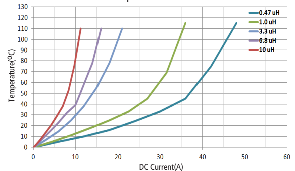
MGV1203 Temperature rise vs DC Current
