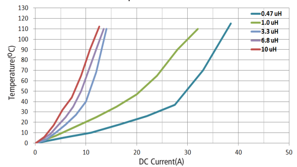
MGV1004 Temperature rise vs DC Current
