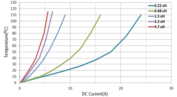
MGV0602 Temperature rise vs DC Current
