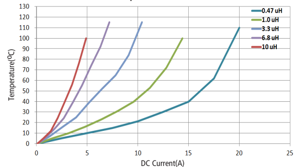
MGV0625 Temperature rise vs DC Current
