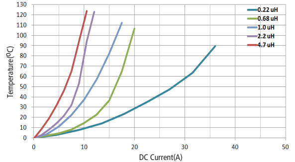
MGV0603 Temperature rise vs DC Current
