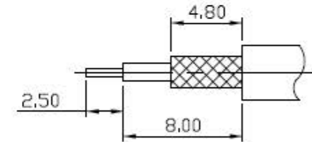
STRIP DIMENSION
